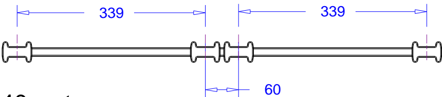
40-er truss
