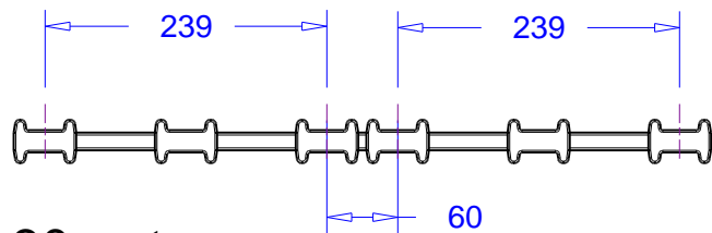
30-er truss
