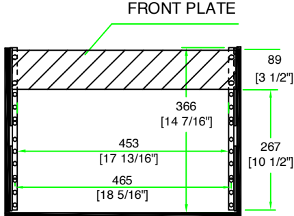
INSIDE VIEW
