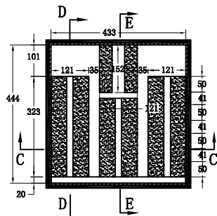
TOP VIEW OF BASE
