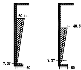
D-D VIEW
