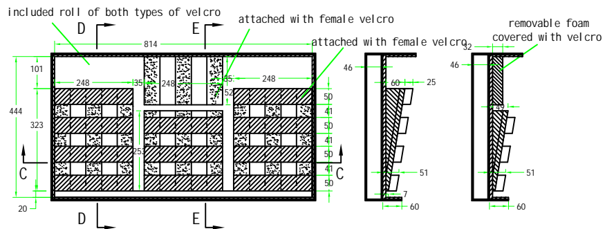
TOP VIEW OF BASE
