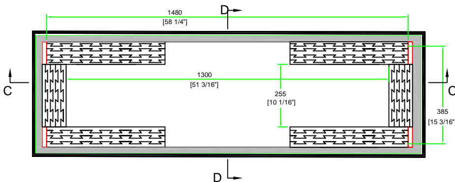
TOP VIEW OF BASE
