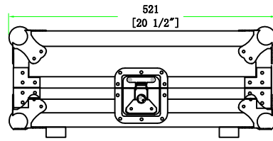
LEFT VIEW
