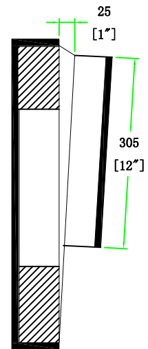
C-C VIEW
