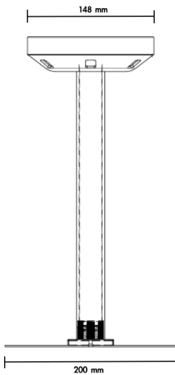
Fixture
