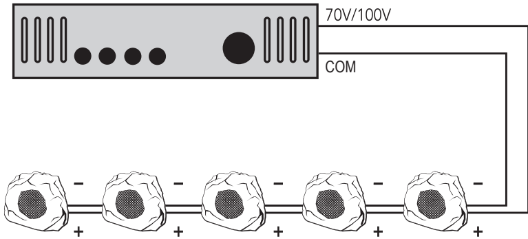
5 speakers connected in parallel using 16W taps
