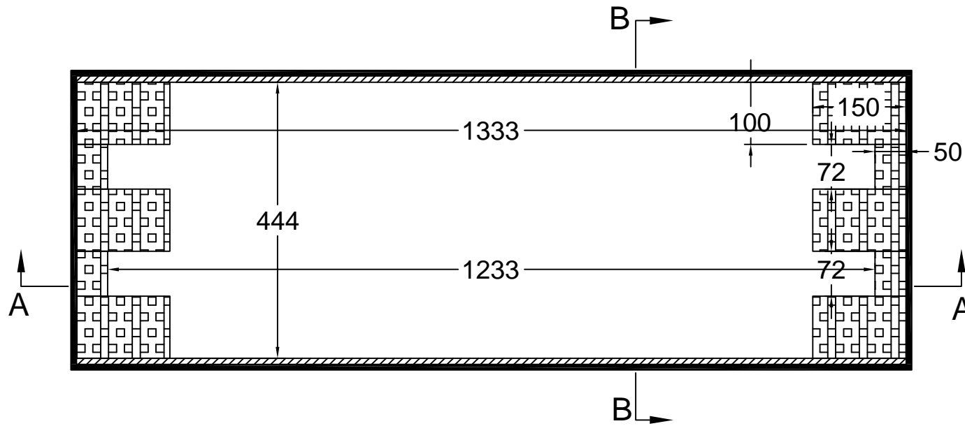
TOP VIEW OF BASE
