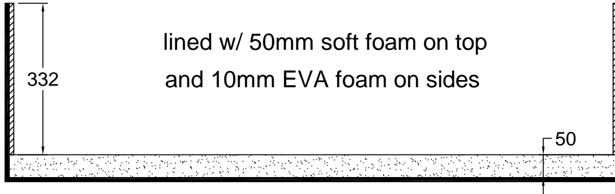
C-C VIEW
