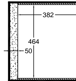
D-D VIEW
