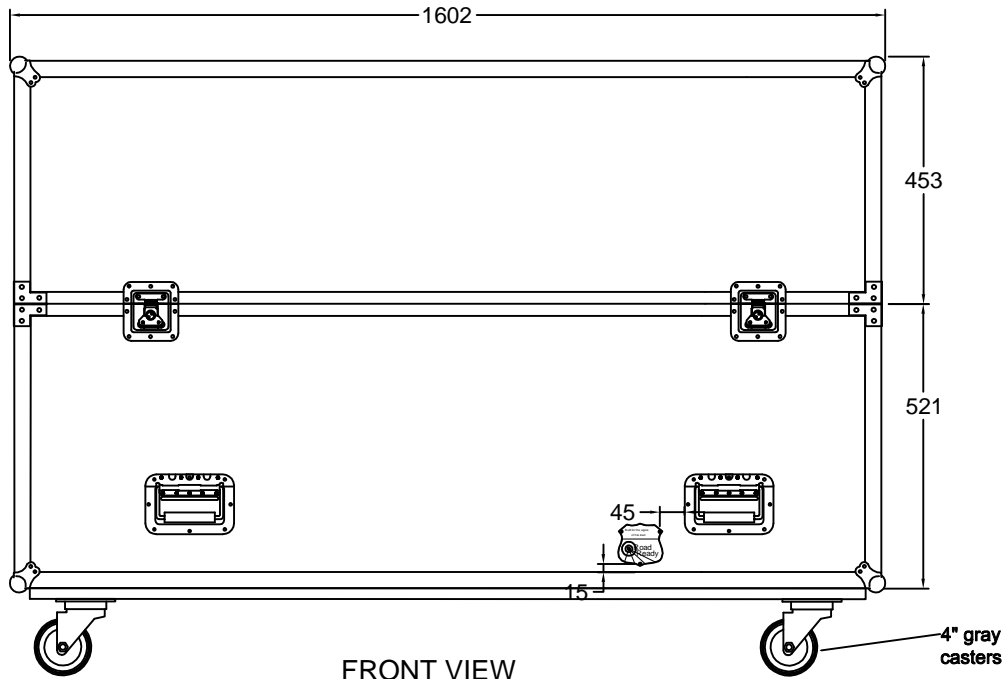
FRONT VIEW BACK VIEW
