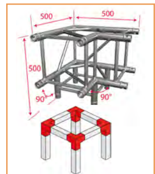
AGQUA-09 Quatro side piece - 3 directions
