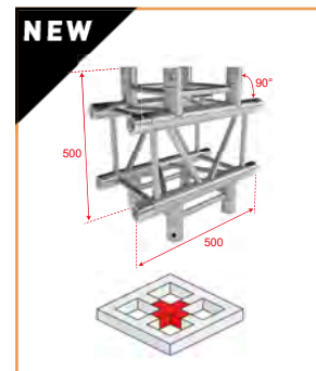
QUATRO-A04 Angle alu square 290 - Heavy duty - 4x 90° directions with sleeves
