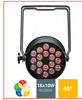
irLED64-18x10FIVEsb PAR64 with 18x10W 5-colour LEDs Black finish
