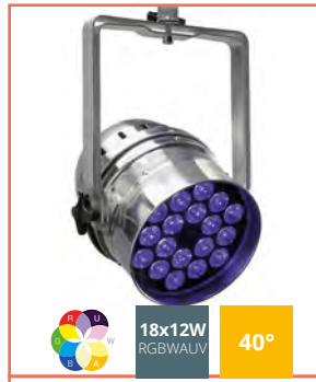
irLED64-18x12SIXss PAR64 with RGBWAUV LEDs - With infrared remote control - Aluminium
