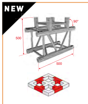
QUATRO-A03 Angle alu square 290 - Heavy duty - 3x 90° directions with sleeves
