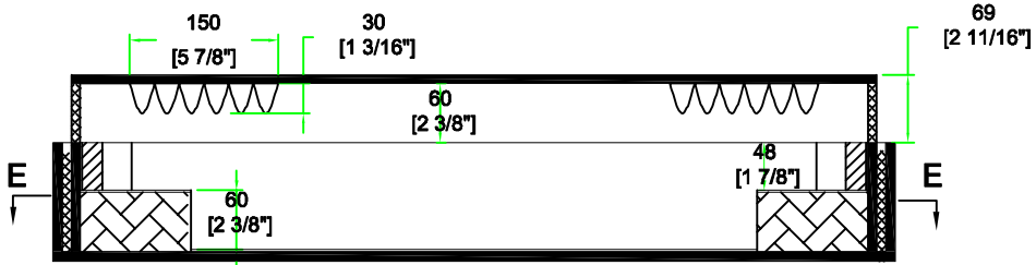
D-D VIEW
