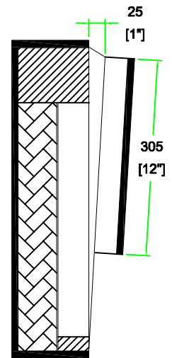
C-C VIEW
