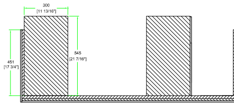
C-C VIEW
