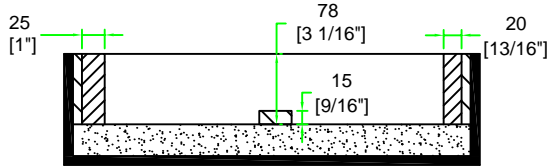
C-C VIEW
