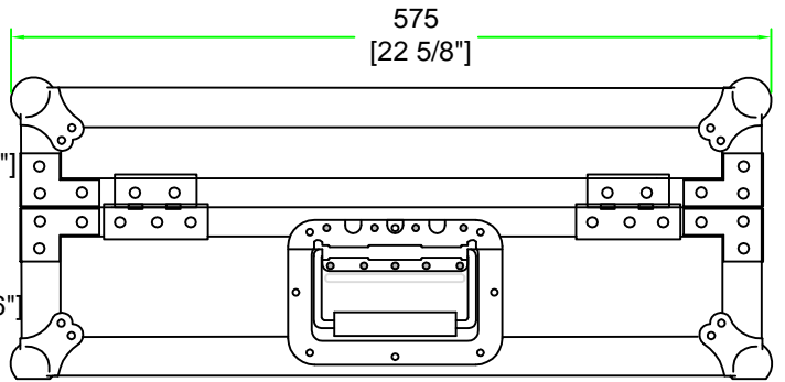
LEFT VIEW
