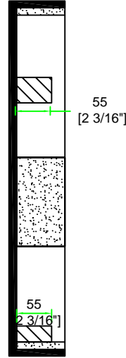
B-B VIEW
