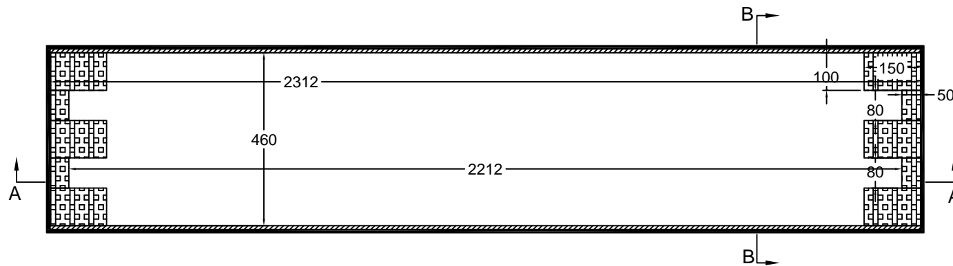
TOP VIEW OF BASE
