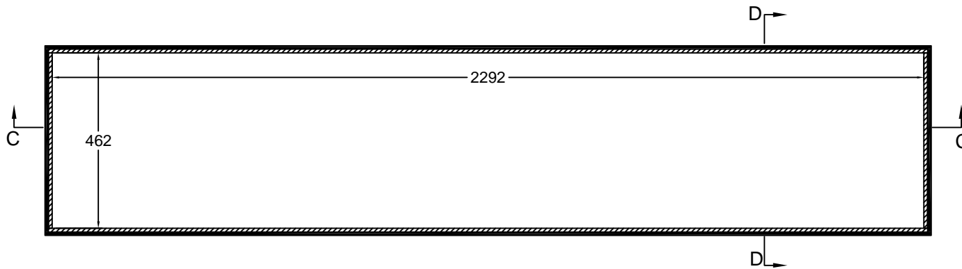
TOP VIEW OF COVER
