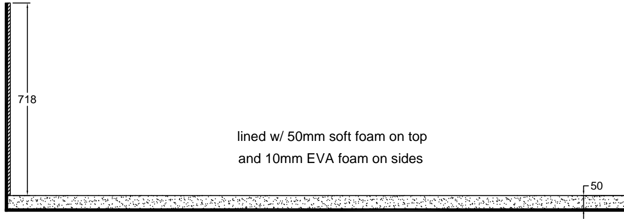
C-C VIEW
