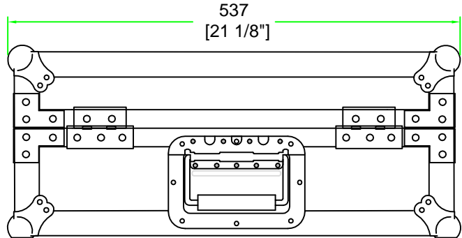
LEFT VIEW
