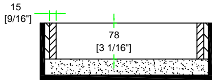
C-C VIEW
