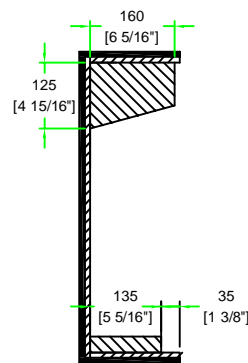
B-B VIEW
