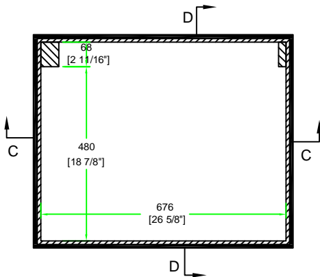
TOP VIEW OF BASE
