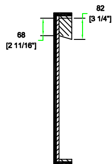
D-D VIEW
