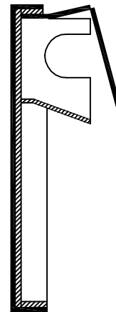
E-E VIEW
